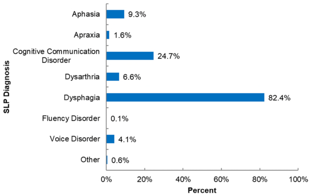
Figure 2: SLP Diagnoses
